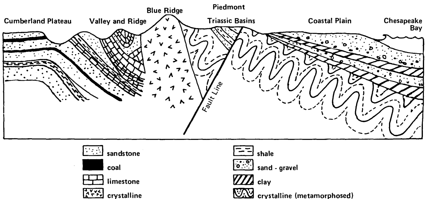
Simplified cross-section of Virginia shows the five provinces: Cumberland Plateau, Valley and Ridge, Blue Ridge, Piedmont (including Triassic Basins), and Coastal Plain. (Used by permission of Lyle Silka, Hydrosystems, Inc.)
